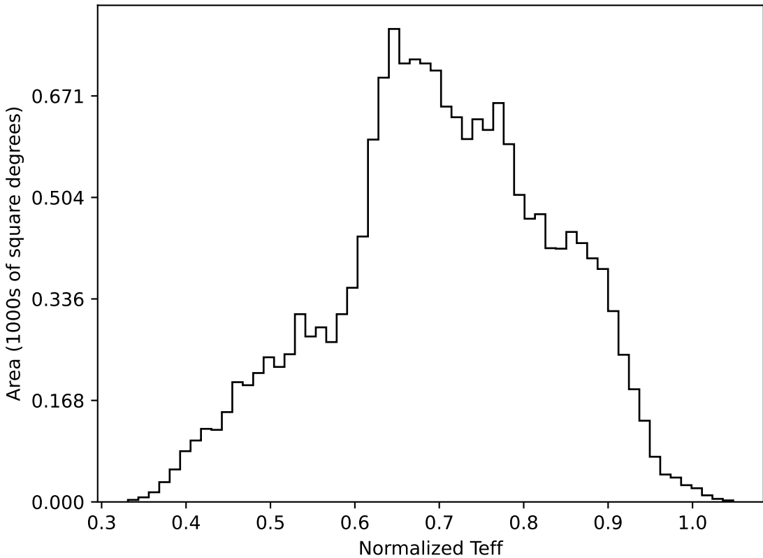
too_elab_r64_d2_griz_v3.4_10yrs WFD all bands: Normalized Teff
