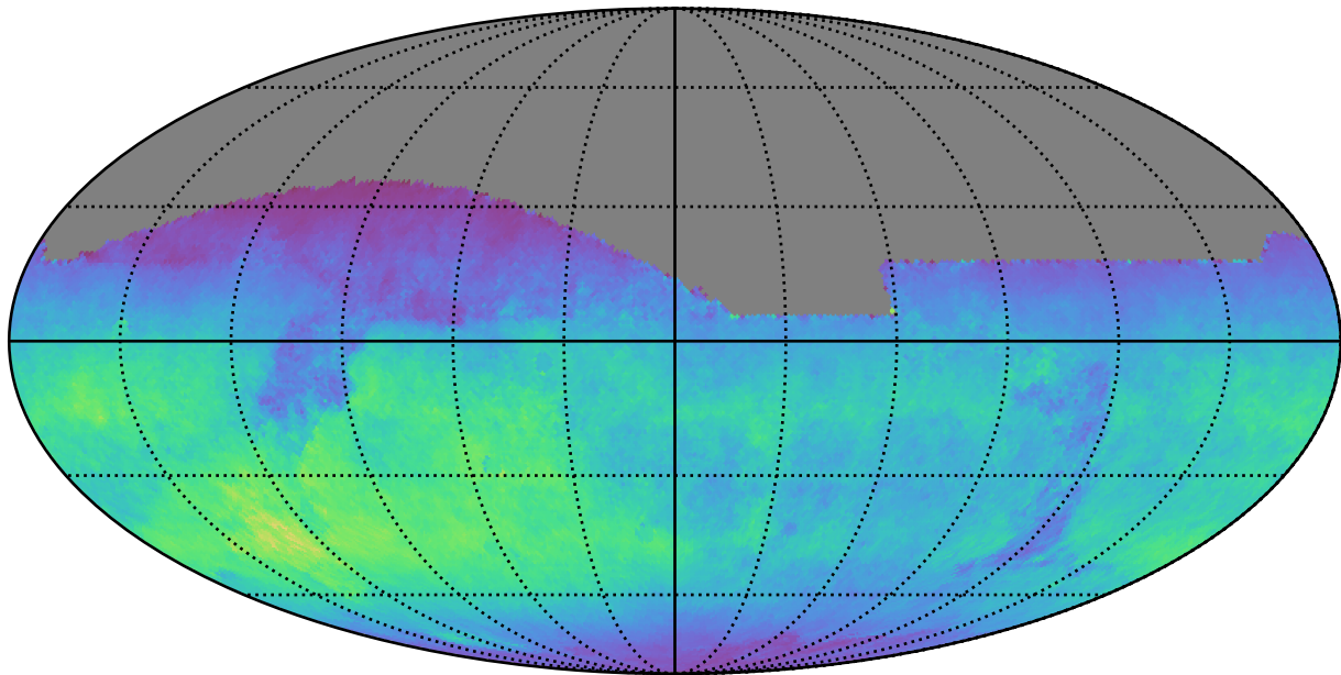
too_elab_r64_d2_griz_v3.4_10yrs All sky z band: Normalized Teff
