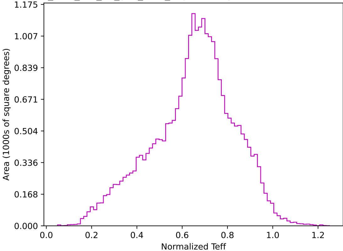
too_elab_r64_d2_griz_v3.4_10yrs All sky z band: Normalized Teff
