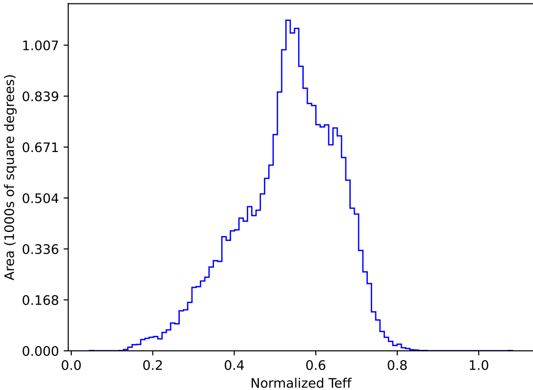
too_elab_r64_d2_griz_v3.4_10yrs All sky y band: Normalized Teff
