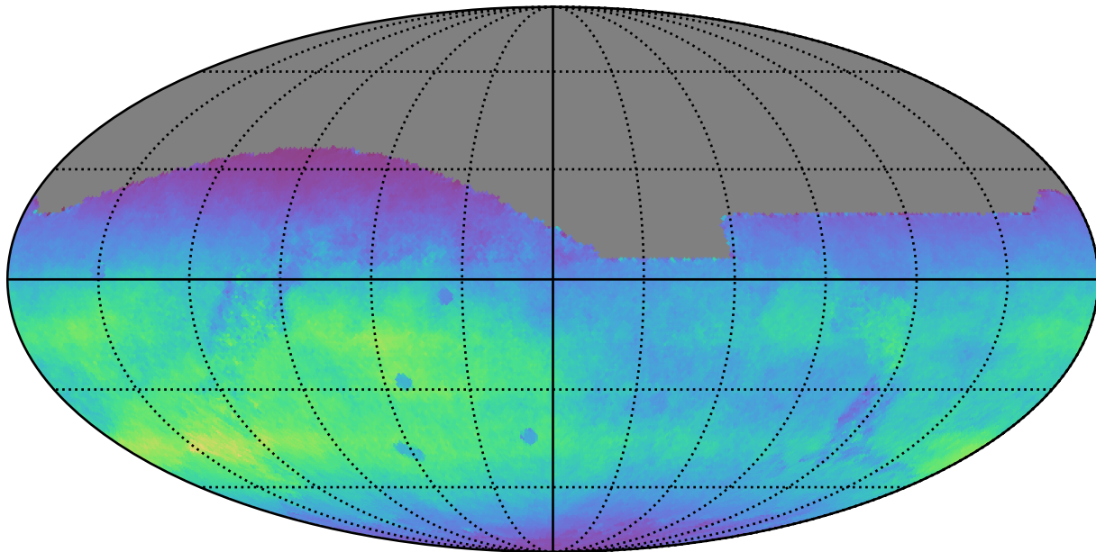
too_elab_r64_d2_griz_v3.4_10yrs All sky r band: Normalized Teff
