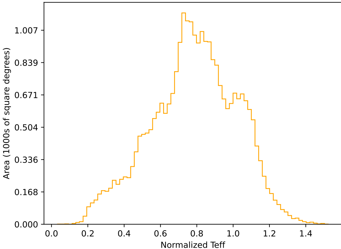
too_elab_r64_d2_griz_v3.4_10yrs All sky r band: Normalized Teff
