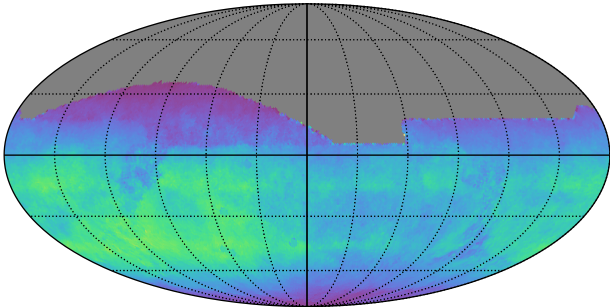
too_elab_r64_d2_griz_v3.4_10yrs All sky i band: Normalized Teff
