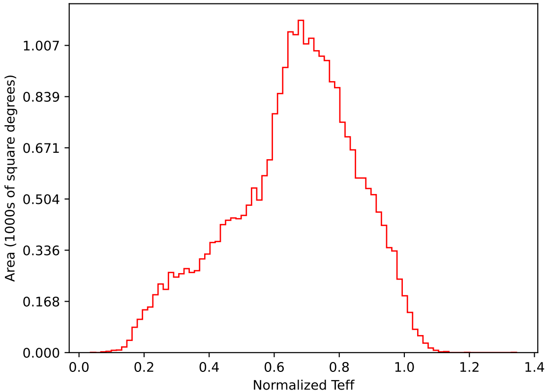
too_elab_r64_d2_griz_v3.4_10yrs All sky i band: Normalized Teff
