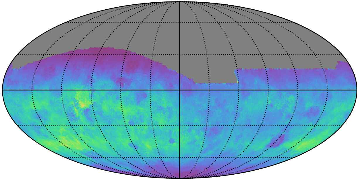
too_elab_r64_d2_griz_v3.4_10yrs All sky g band: Normalized Teff
