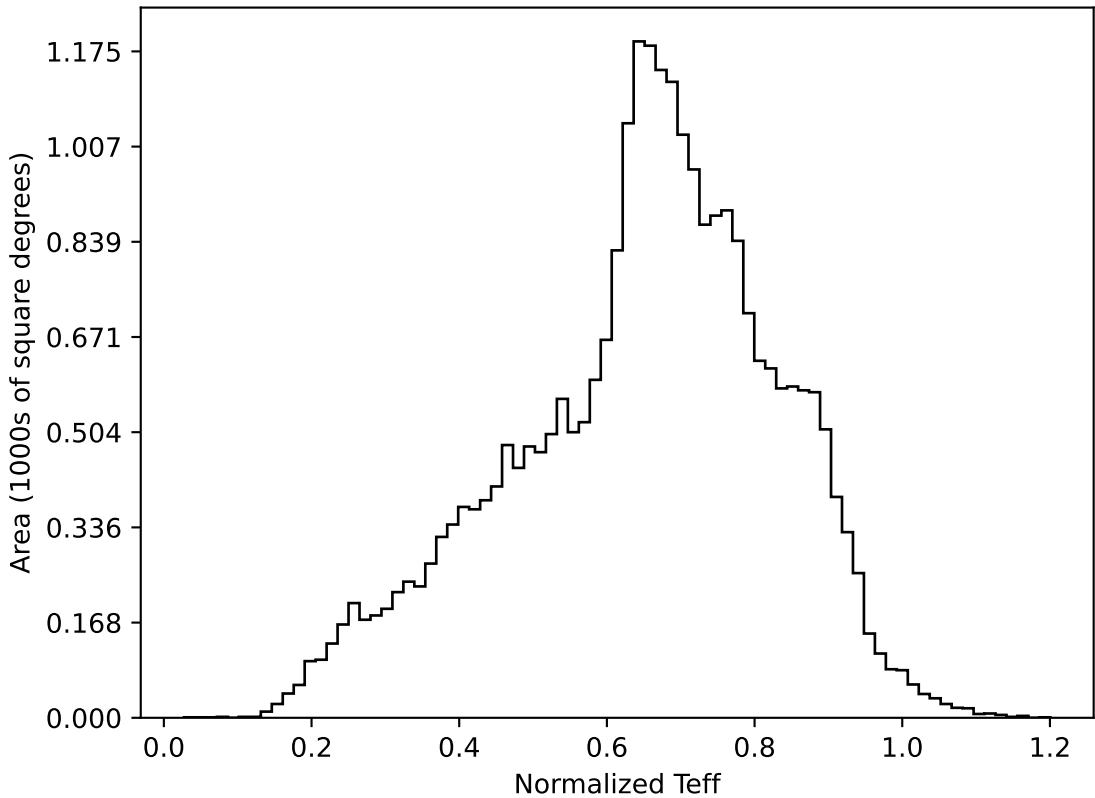
too_elab_r64_d2_griz_v3.4_10yrs All sky all bands: Normalized Teff
