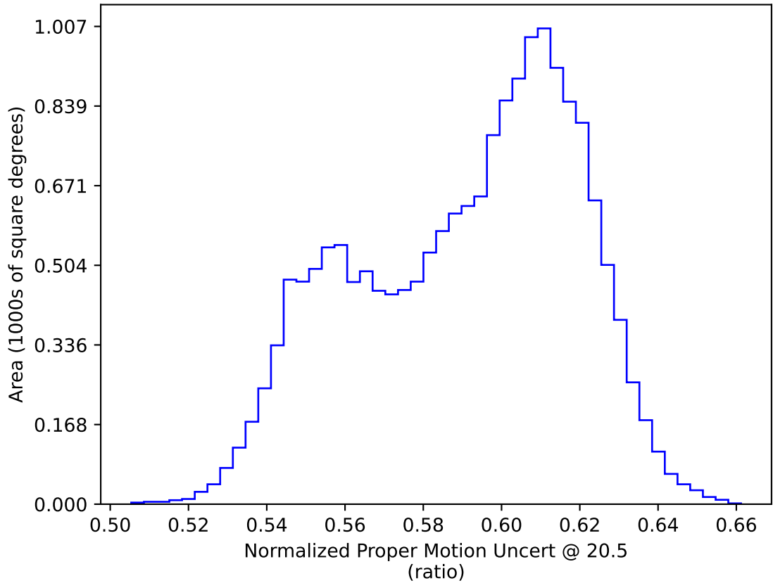
too_elab_r64_d2_griz_v3.4_10yrs WFD: Normalized Proper Motion Uncert @ 20.5
