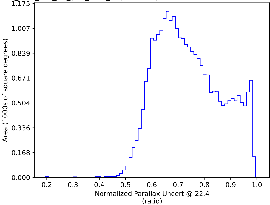
too_elab_r64_d2_griz_v3.4_10yrs All sky: Normalized Parallax Uncert @ 22.4
