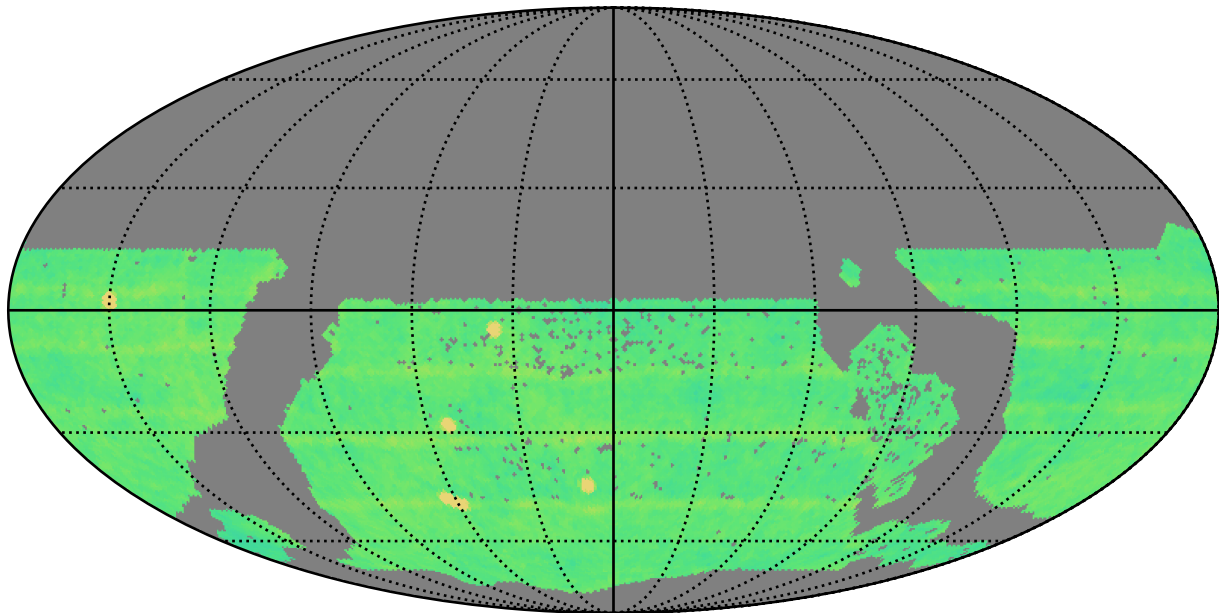
too_elab_r64_d2_griz_v3.4_10yrs WFD all bands: N Unique Nights
