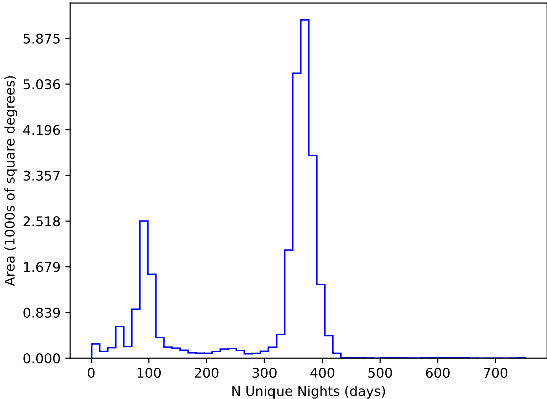
too_elab_r64_d2_griz_v3.4_10yrs All sky all bands: N Unique Nights
