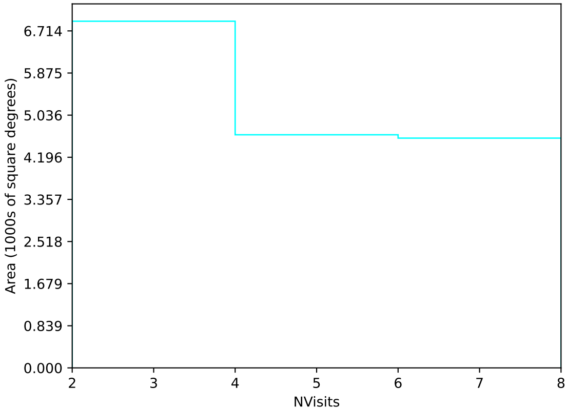
too_elab_r64_d2_griz_v3.4_10yrs Yr 3-4 u band: NVisits
