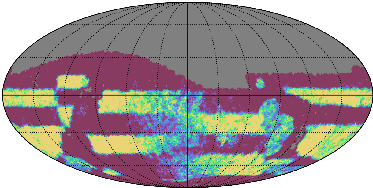
too_elab_r64_d2_griz_v3.4_10yrs Yr 3-4 r band: NVisits
