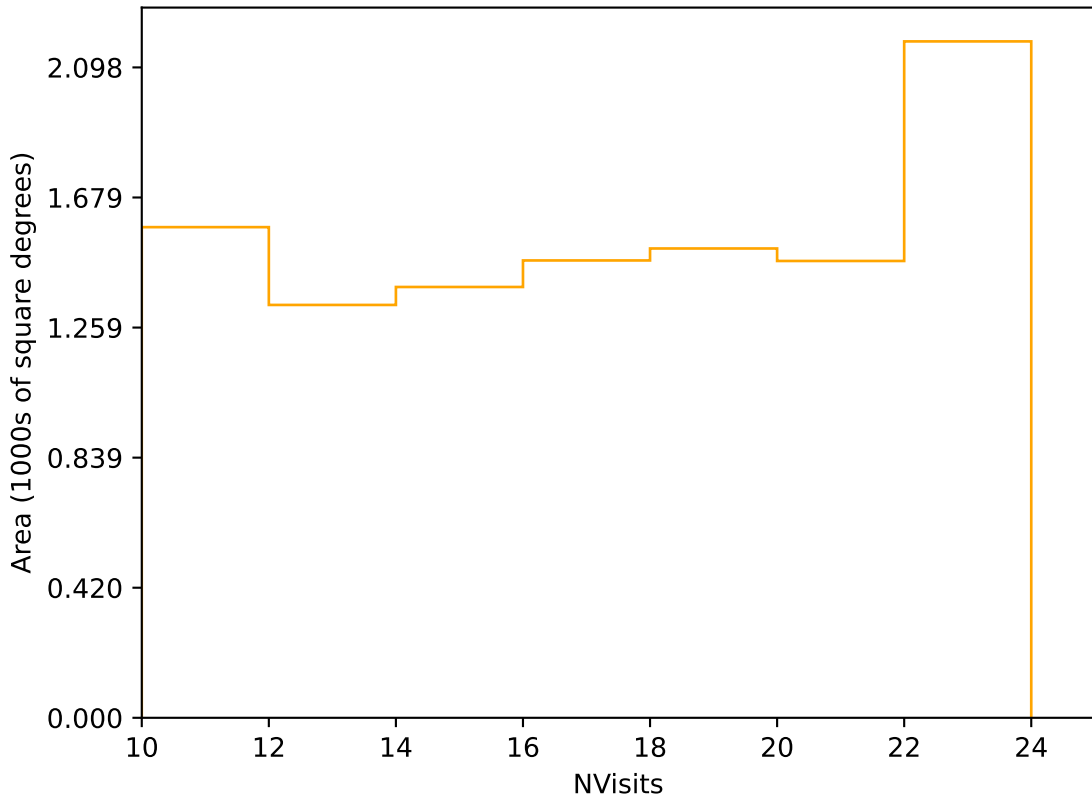
too_elab_r64_d2_griz_v3.4_10yrs Yr 3-4 r band: NVisits
