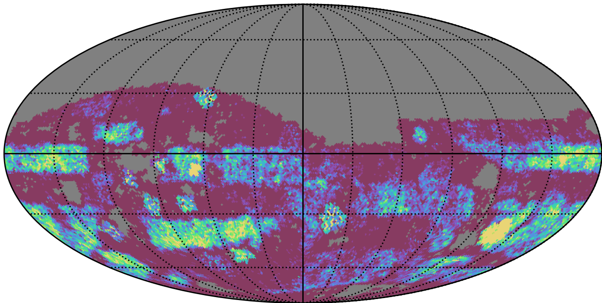
too_elab_r64_d2_griz_v3.4_10yrs Yr 3-4 g band: NVisits
