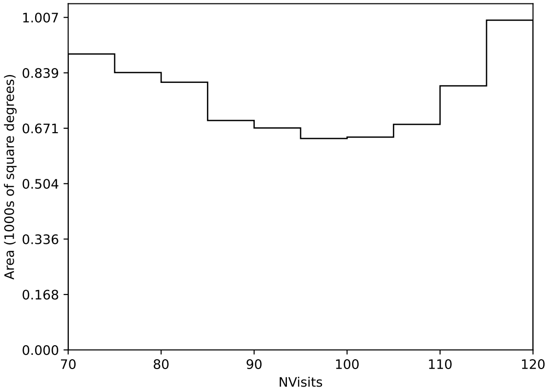
too_elab_r64_d2_griz_v3.4_10yrs Yr 3-4 all bands: NVisits
