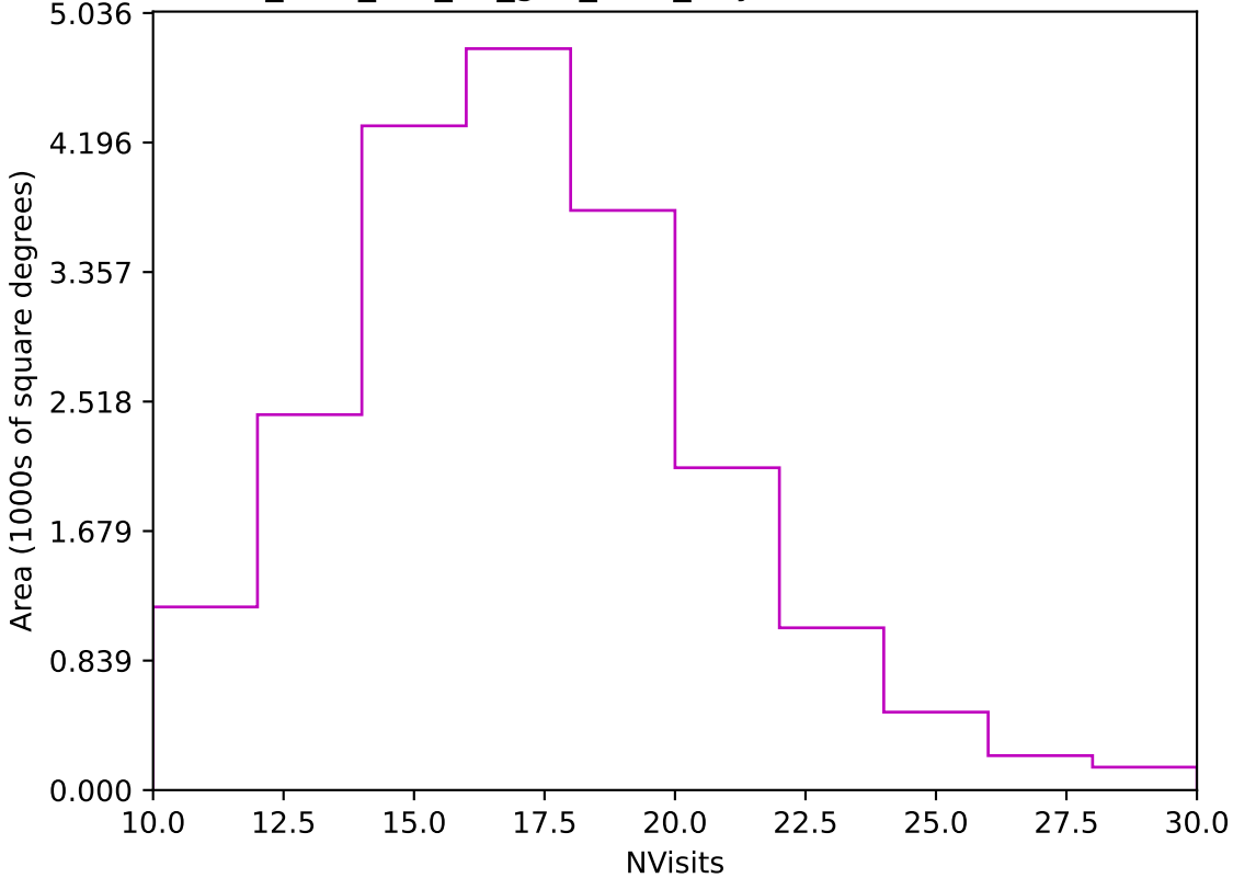
too_elab_r64_d2_griz_v3.4_10yrs Yr 1 z band: NVisits
