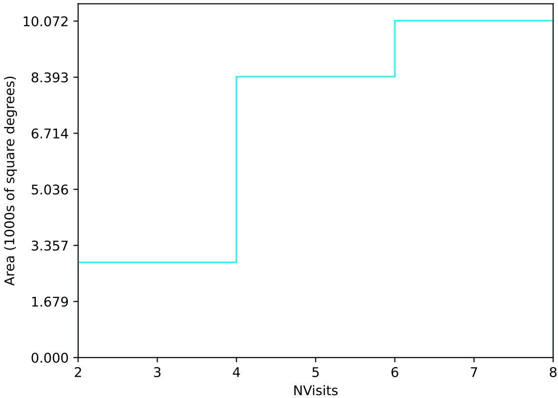
too_elab_r64_d2_griz_v3.4_10yrs Yr 1 u band: NVisits
