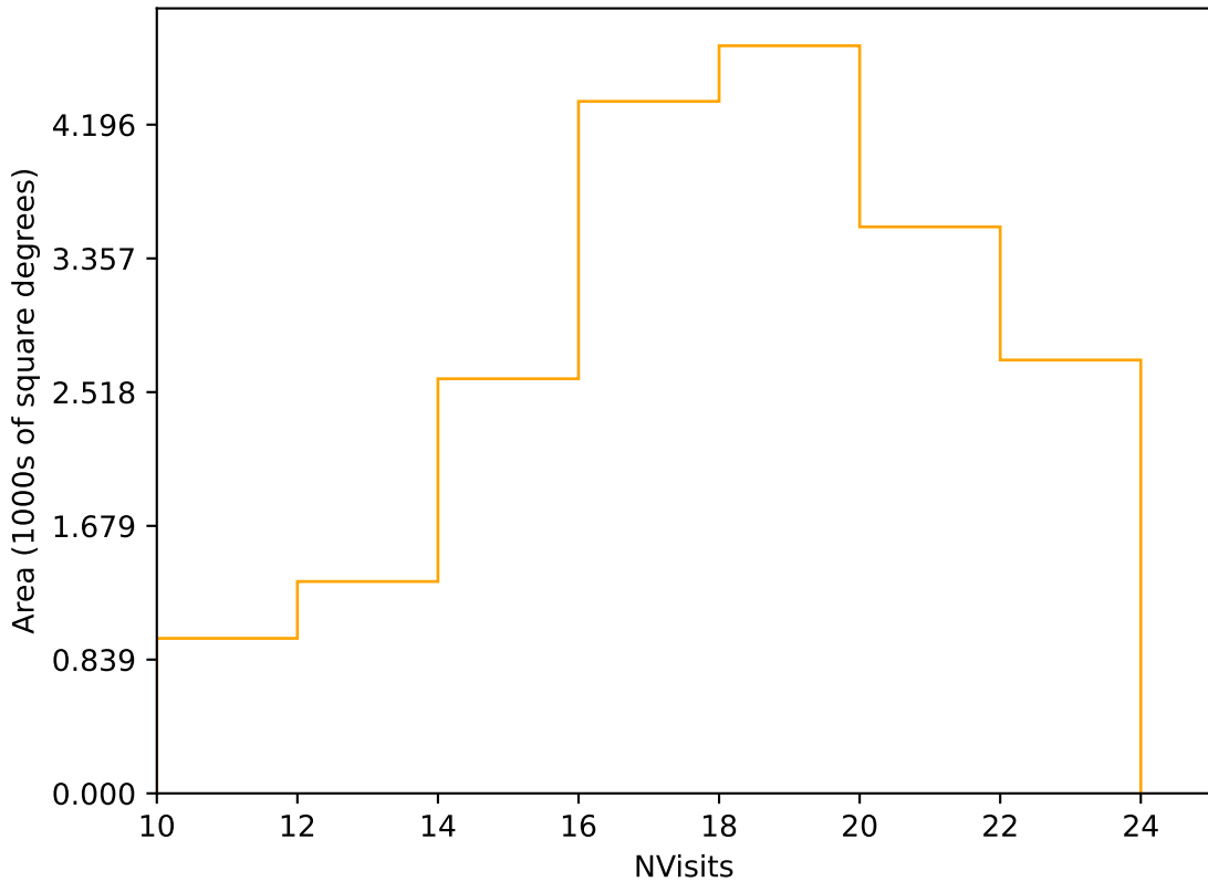
too_elab_r64_d2_griz_v3.4_10yrs Yr 1 r band: NVisits
