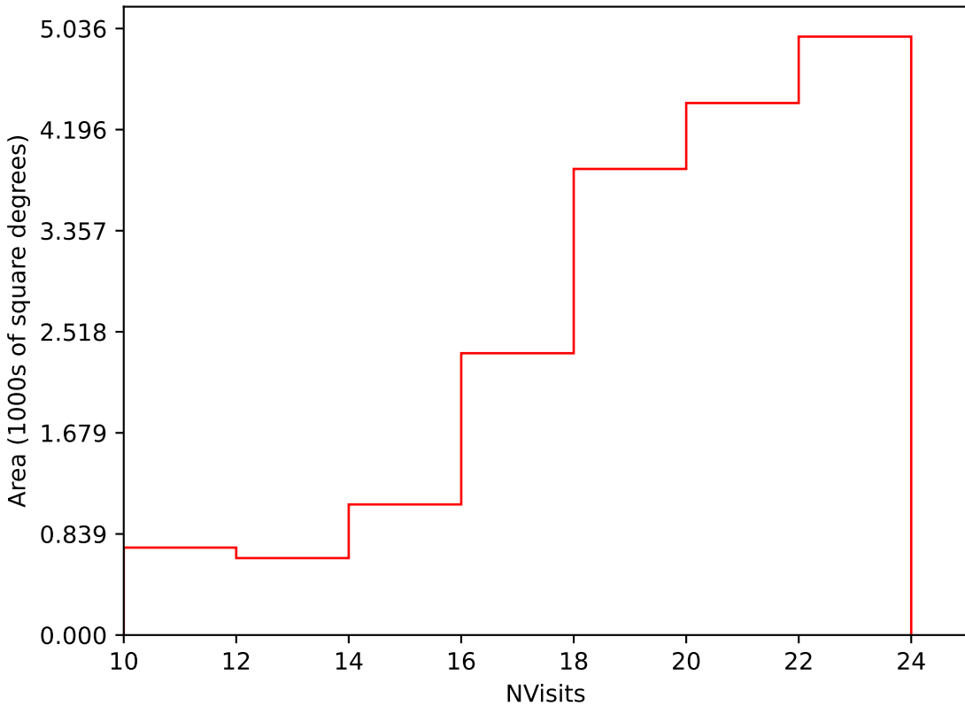
too_elab_r64_d2_griz_v3.4_10yrs Yr 1 i band: NVisits
