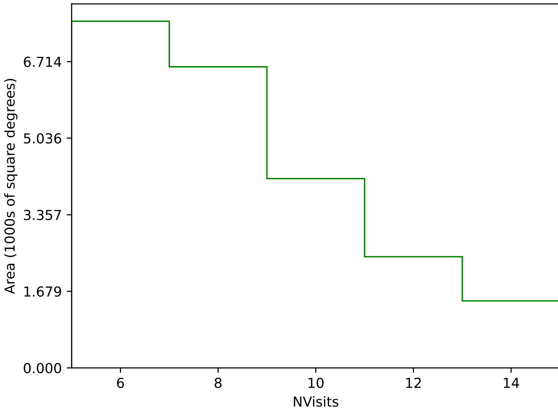
too_elab_r64_d2_griz_v3.4_10yrs Yr 1 g band: NVisits
