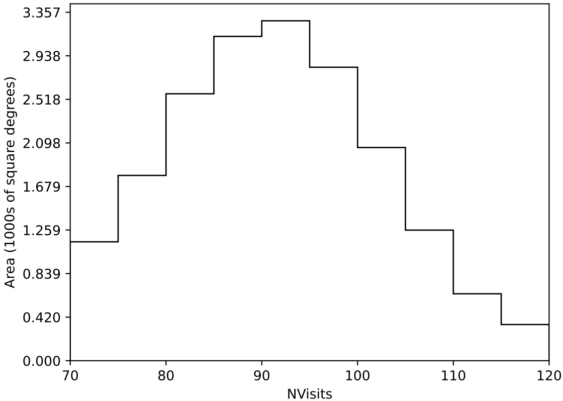
too_elab_r64_d2_griz_v3.4_10yrs Yr 1 all bands: NVisits
