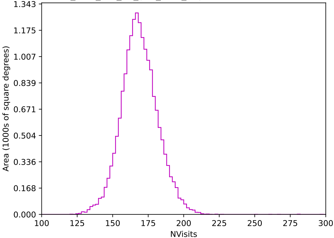
too_elab_r64_d2_griz_v3.4_10yrs WFD z band: NVisits
