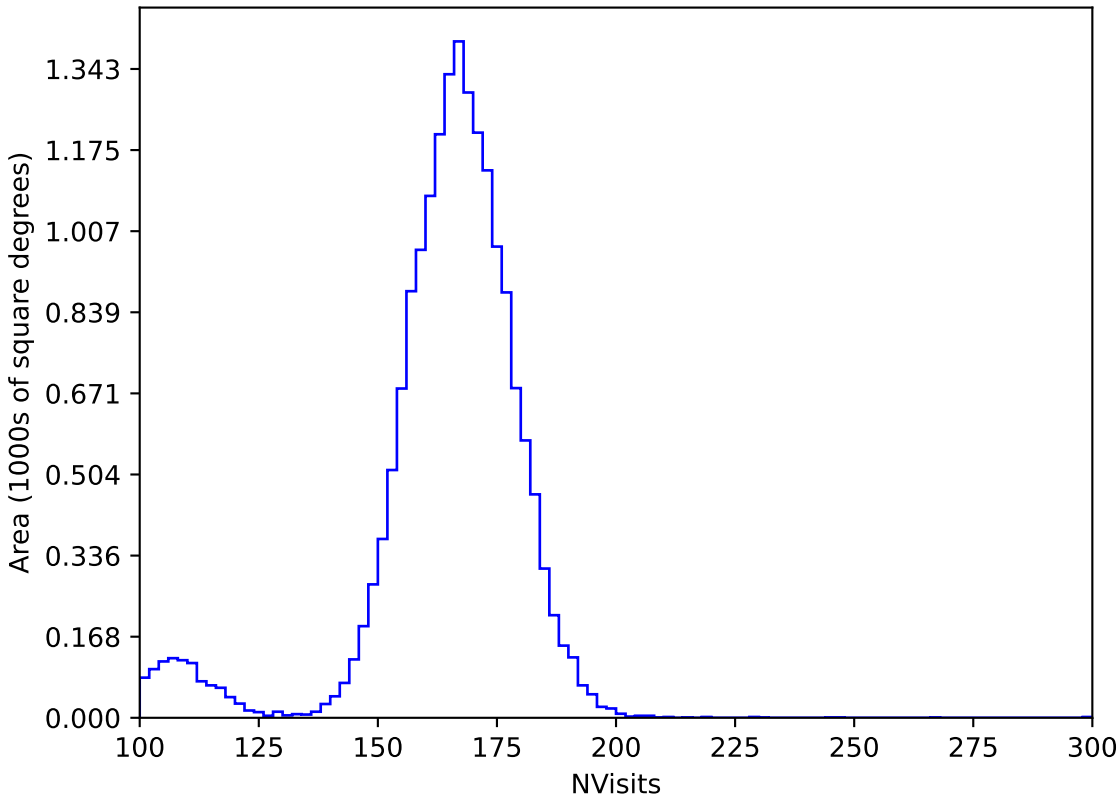
too_elab_r64_d2_griz_v3.4_10yrs WFD y band: NVisits
