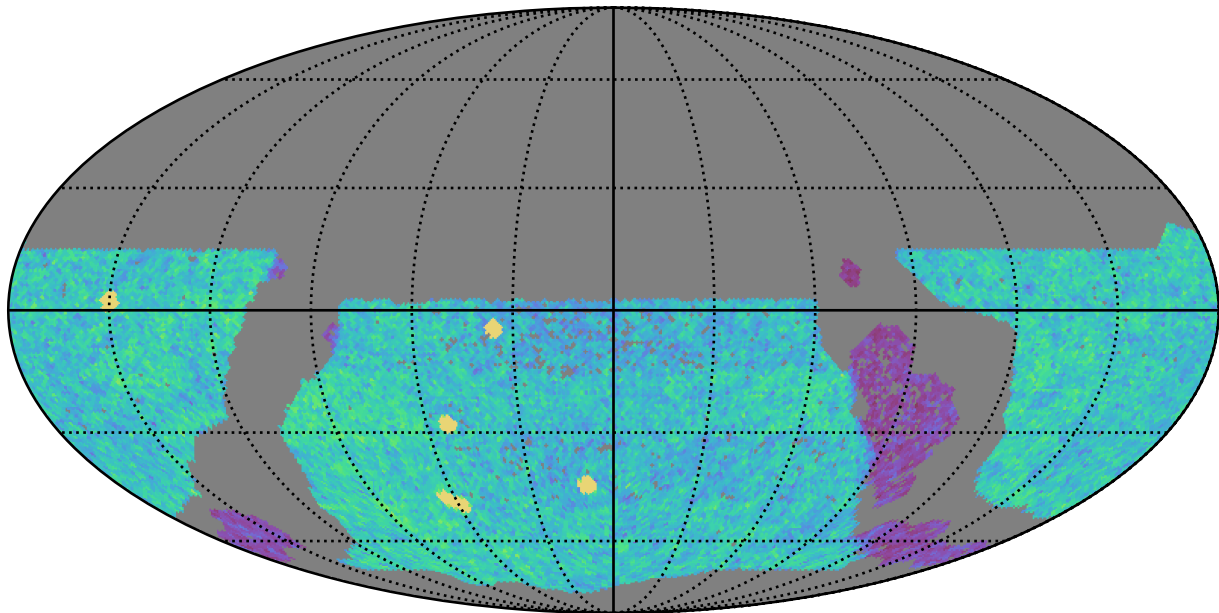
too_elab_r64_d2_griz_v3.4_10yrs WFD u band: NVisits
