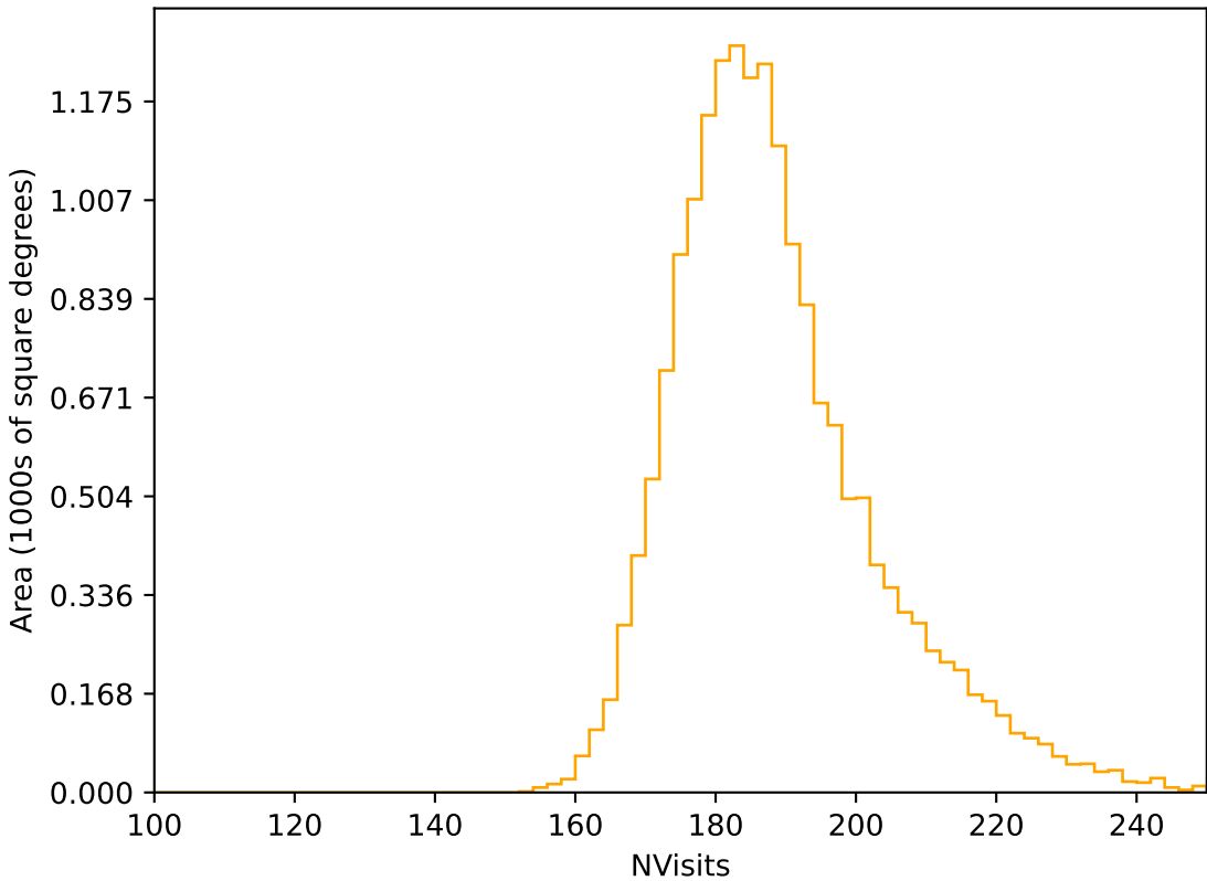
too_elab_r64_d2_griz_v3.4_10yrs WFD r band: NVisits
