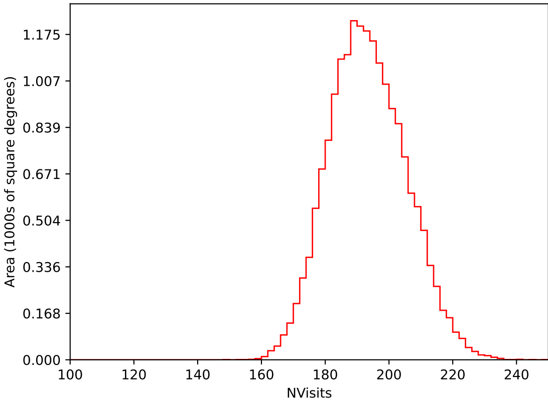
too_elab_r64_d2_griz_v3.4_10yrs WFD i band: NVisits
