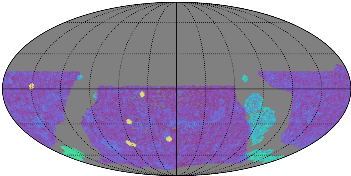
too_elab_r64_d2_griz_v3.4_10yrs WFD g band: NVisits
