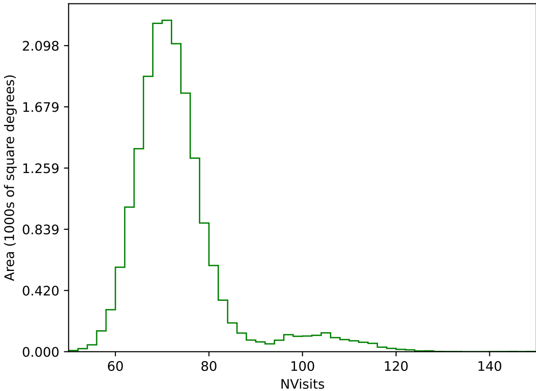
too_elab_r64_d2_griz_v3.4_10yrs WFD g band: NVisits
