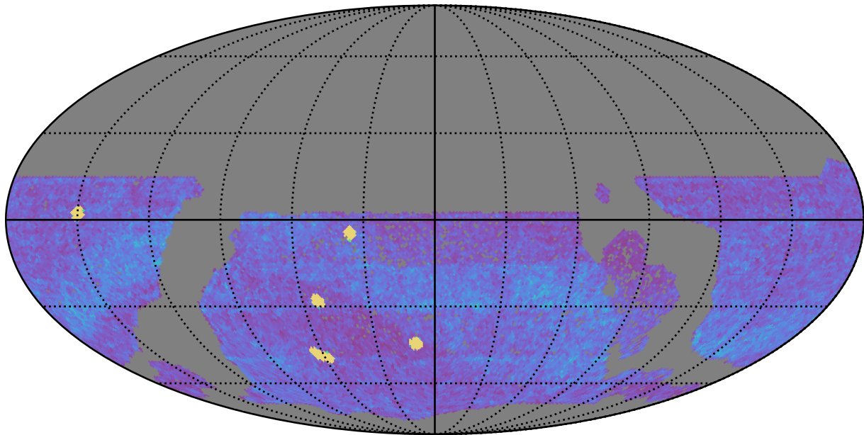
too_elab_r64_d2_griz_v3.4_10yrs WFD all bands: NVisits
