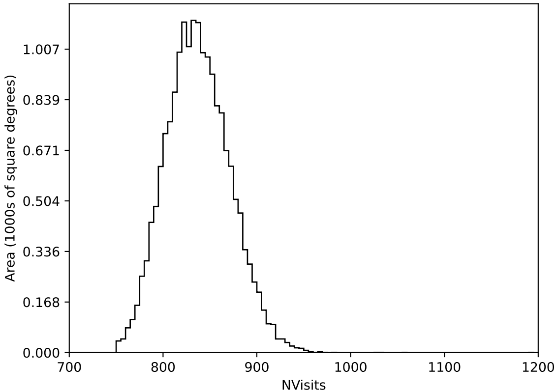
too_elab_r64_d2_griz_v3.4_10yrs WFD all bands: NVisits
