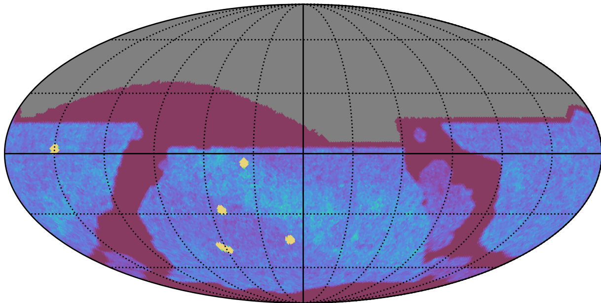
too_elab_r64_d2_griz_v3.4_10yrs All sky z band: NVisits
