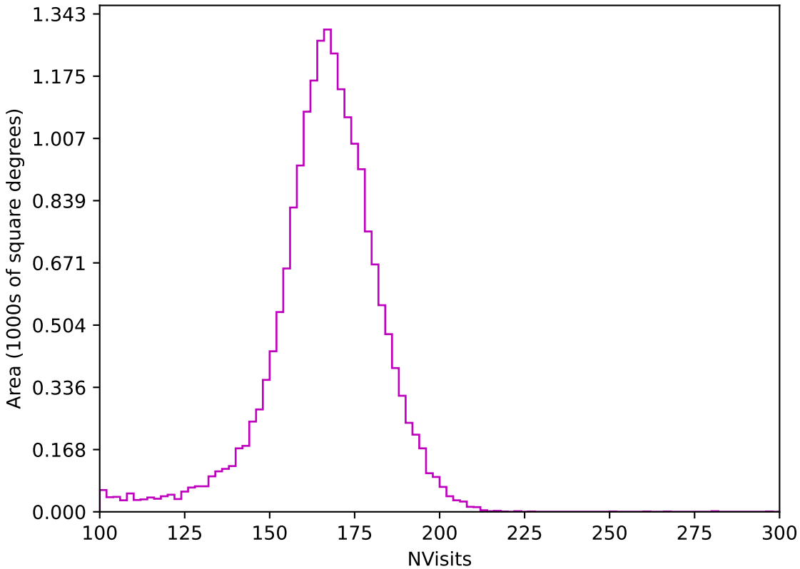
too_elab_r64_d2_griz_v3.4_10yrs All sky z band: NVisits
