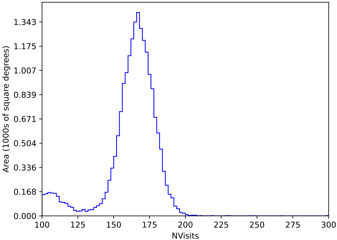
too_elab_r64_d2_griz_v3.4_10yrs All sky y band: NVisits
