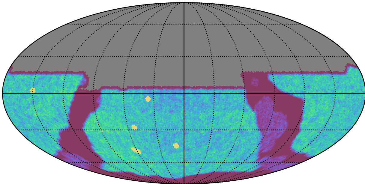
too_elab_r64_d2_griz_v3.4_10yrs All sky u band: NVisits
