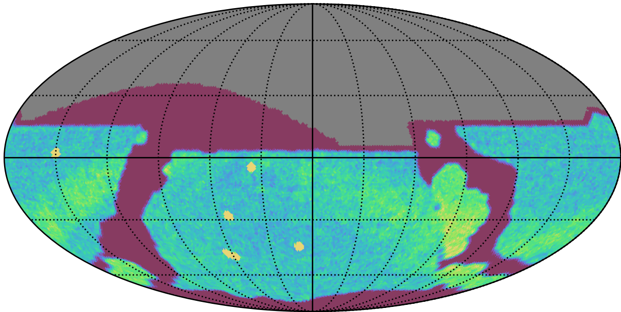
too_elab_r64_d2_griz_v3.4_10yrs All sky r band: NVisits
