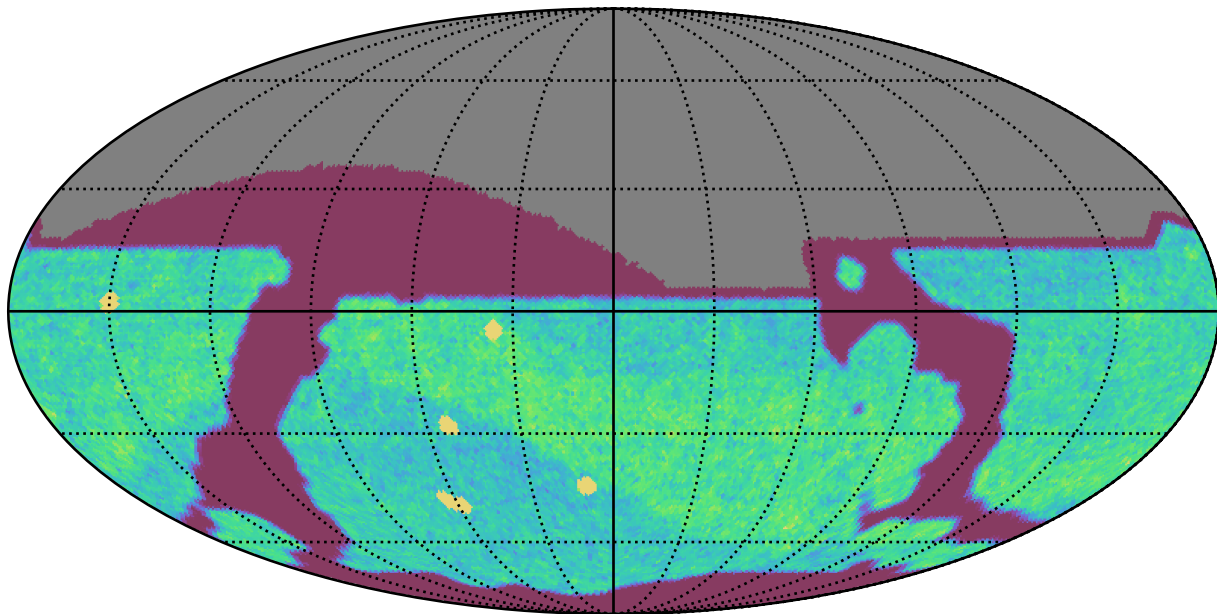
too_elab_r64_d2_griz_v3.4_10yrs All sky i band: NVisits
