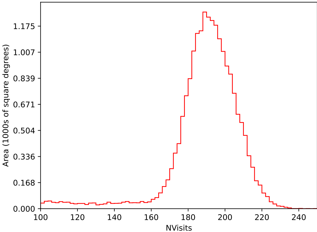
too_elab_r64_d2_griz_v3.4_10yrs All sky i band: NVisits
