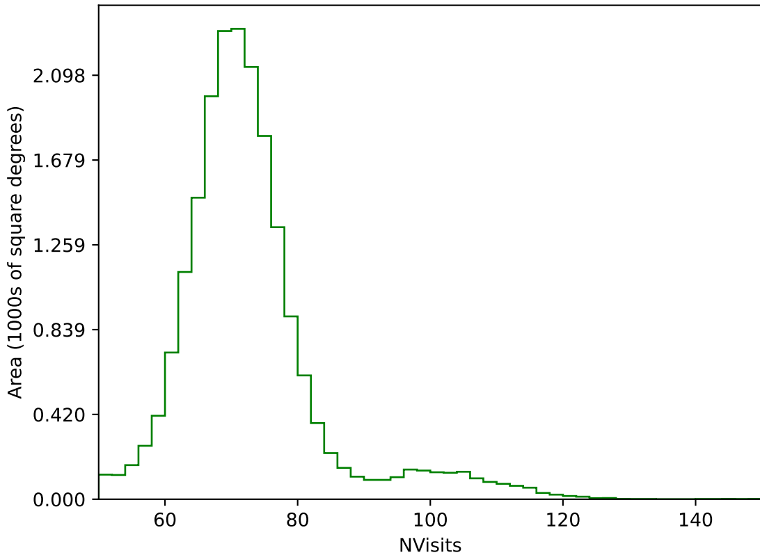
too_elab_r64_d2_griz_v3.4_10yrs All sky g band: NVisits
