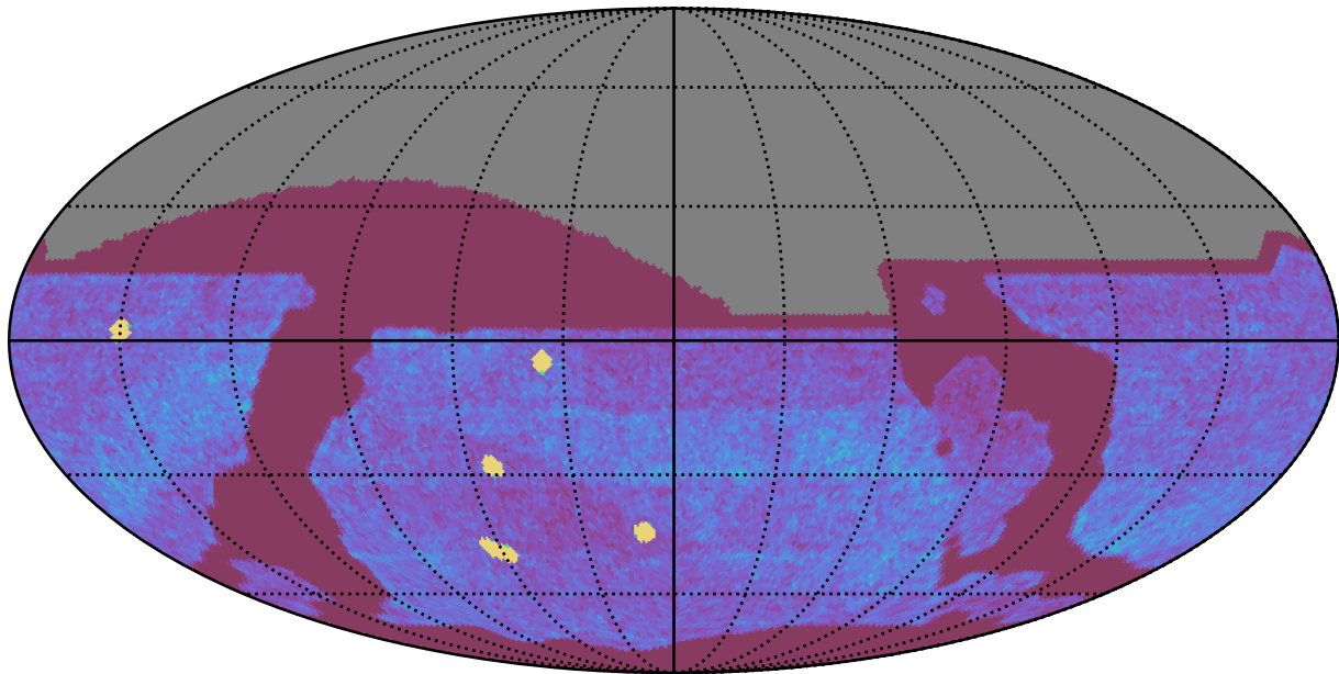
too_elab_r64_d2_griz_v3.4_10yrs All sky all bands: NVisits
