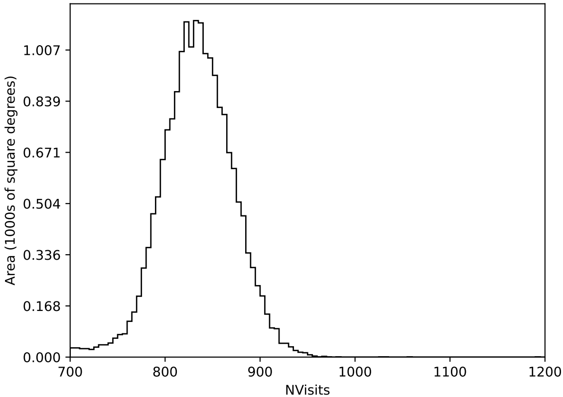
too_elab_r64_d2_griz_v3.4_10yrs All sky all bands: NVisits
