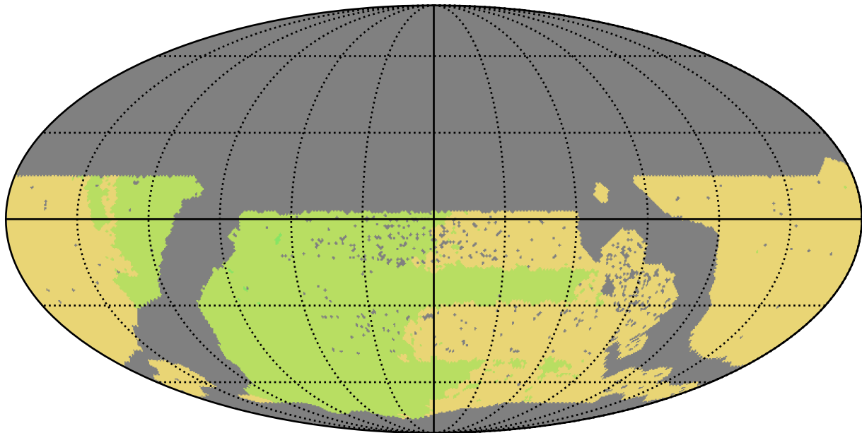
too_elab_r64_d2_griz_v3.4_10yrs WFD all bands: NSeasons
