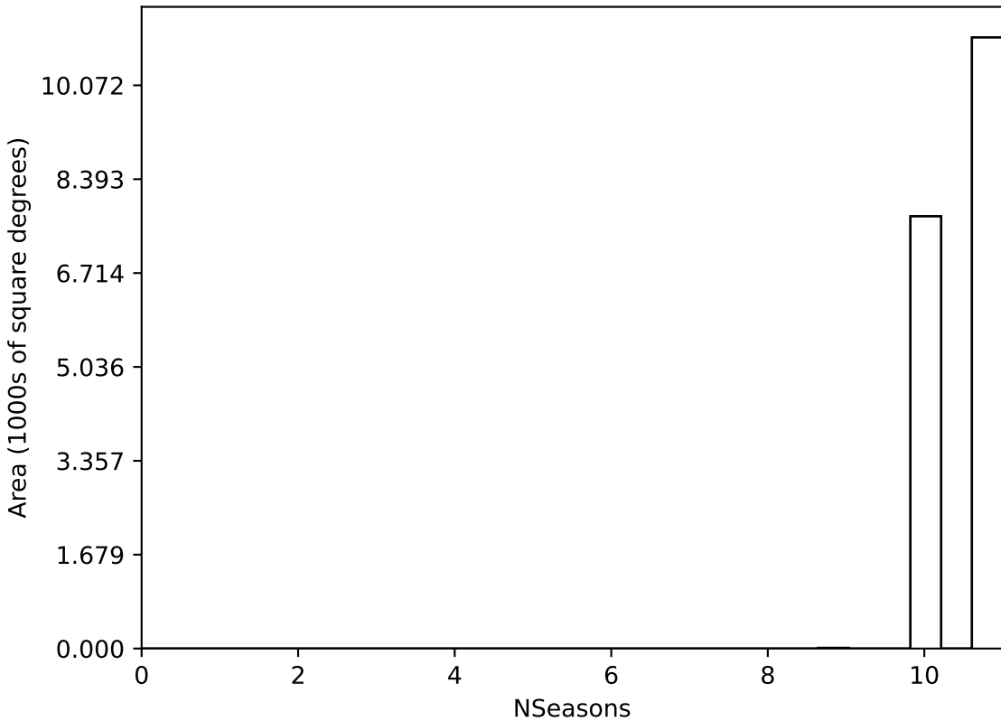
too_elab_r64_d2_griz_v3.4_10yrs WFD all bands: NSeasons
