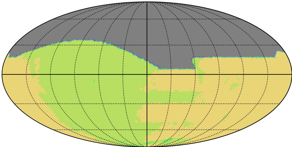
too_elab_r64_d2_griz_v3.4_10yrs All sky all bands: NSeasons
