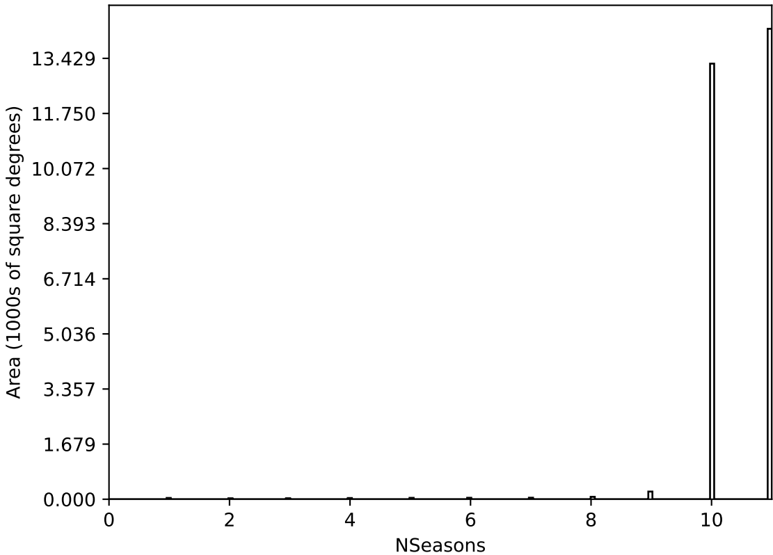
too_elab_r64_d2_griz_v3.4_10yrs All sky all bands: NSeasons
