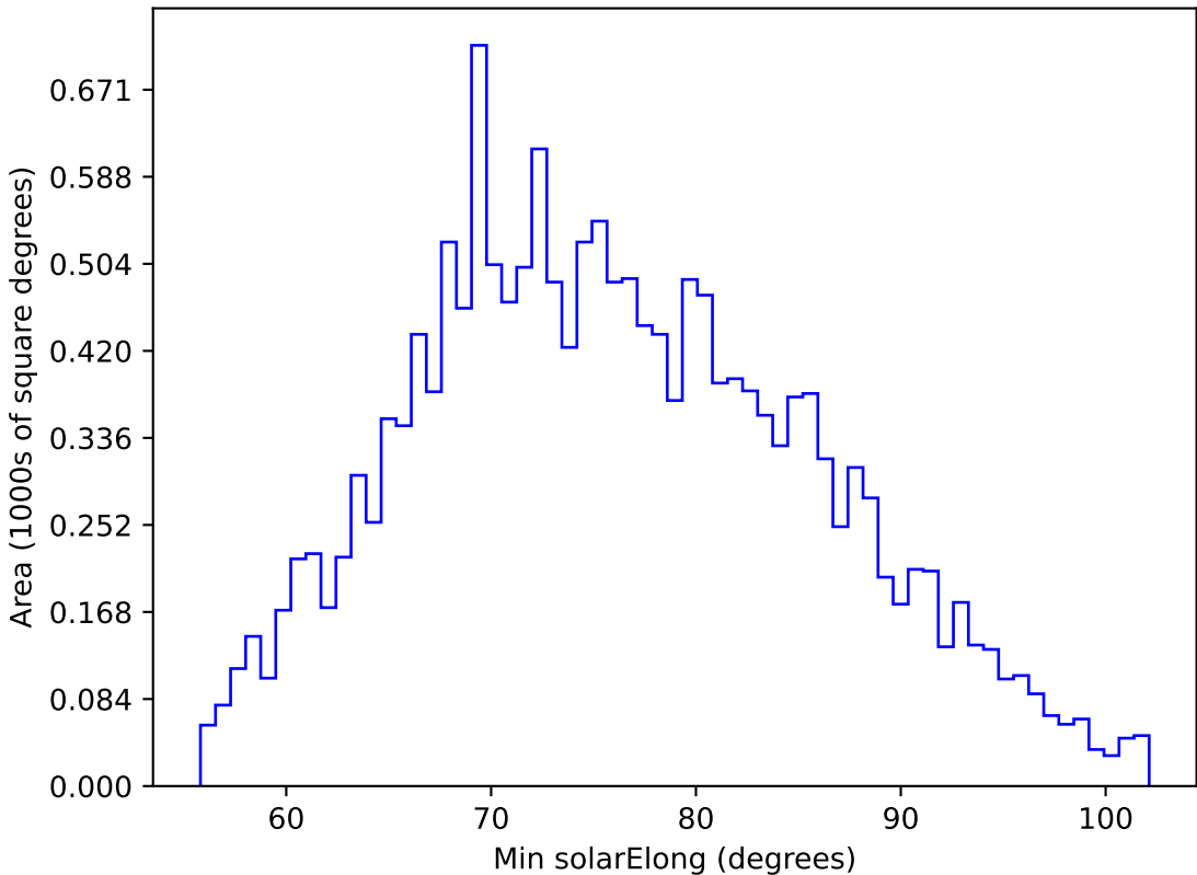
too_elab_r64_d2_griz_v3.4_10yrs WFD u band: Min solarElong
