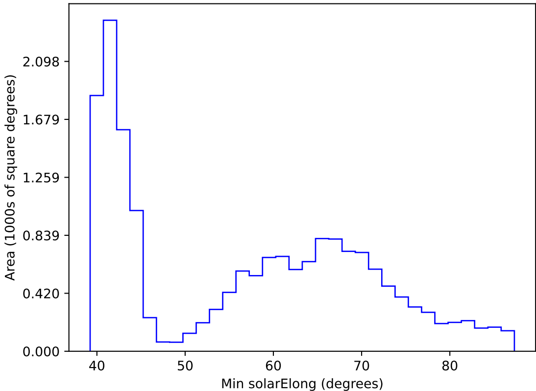
too_elab_r64_d2_griz_v3.4_10yrs WFD r band: Min solarElong
